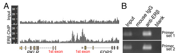
Fig. 10. ERβ-binding profiles for human FDPS and ChIP assay for mouse Fdps gene. (A) ChIP-seq data for doxycycline-inducible ERβ-expressing human MDA-MB-231 cells treated with estradiol was obtained from the GEO database (accession no. GSE108981). Peaks in ERβ ChIP profiles indicate ERβ binding to the region. FDPS showed peaks around the first exons in ERβ ChIP profile, whereas the negative control input profile (DNAs from chromatin before ChIP) did not show the peak. As an additional negative control, the PKLR gene, near the FDPS gene, did not have a peak. (B) ERβ binds to the putative ERE of mouse Fdps gene. ChIP using normal mouse IgG and anti-ERβ was performed for the chromatin isolated from mouse N20.1 oligodendrocyte cell line (21) treated with ERβ ligand (DPN). Two sets of primers were designed across the region containing putative ERE of Fdps gene (51).
